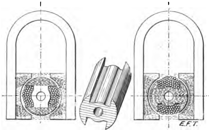
FIG. 338. —Diagram of the Construction and Theoretical Operation of a Typical Magneto-generator. Between the prongs of the horseshoe magnets, the shuttle-shaped armature is wound from end to end with insulated wire, so that when rotated a powerful current is produced in the windings by cutting the magnetic lines, whose varying strength is shown by the shaded portions in the two views. When the armature is in the position shown in the first diagram, the lines of force mostly converge at the top and bottom, finding a direct path through the metal end flanges of the shuttle. When in the position shown in the second diagram, the lines are converged so as to pass through the metallic core of the armature; the most direct path being chosen in both cases.
